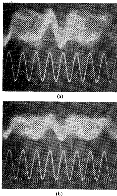
Fig. 5. Carrier and demodulated output. (a) Without optical attenuation. (b) With approximately 30 percent attenuation.
